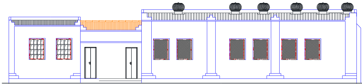
FACHADA PRINCIPAL
